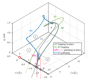
Figure 2: Connected (Conservative) Gaits
